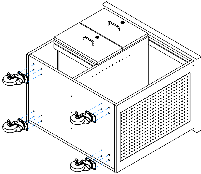
DOOR AND BOTTOM DRAWER REMOVED TO SHOW CLARITY
